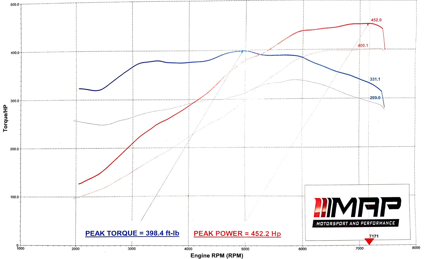
Peak Torque* and Hp* vs. RPM
