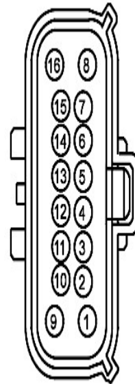
FEMALE Harness 14290
